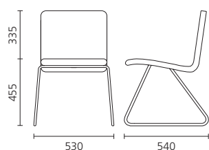
Side chair
