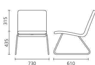
Lounge chair
